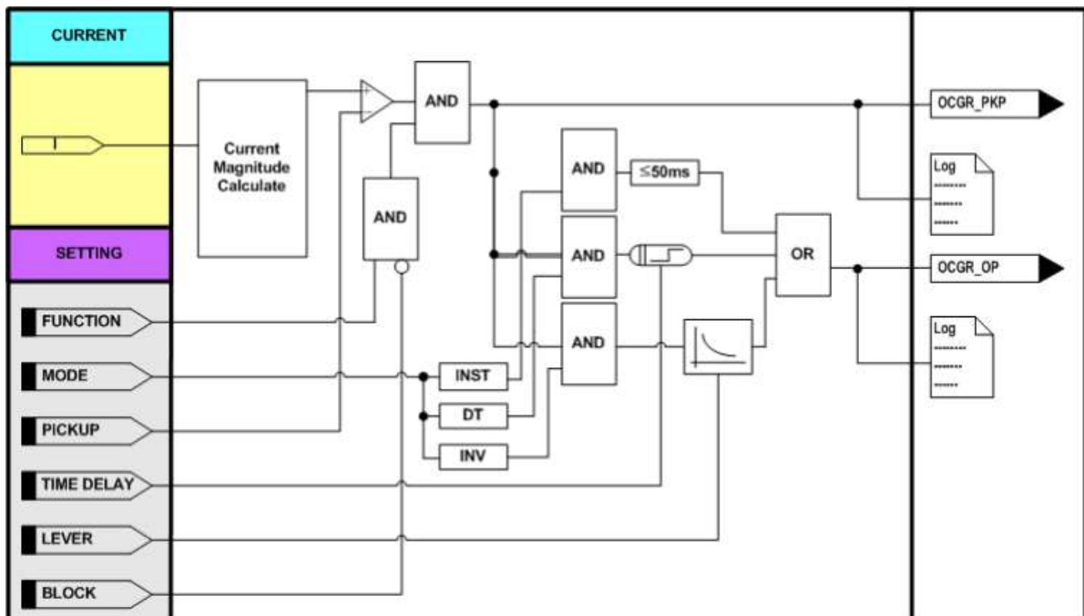
<Figure. 지락과전류 (OCGR) 1 ~ 3 Logic Diagram>
